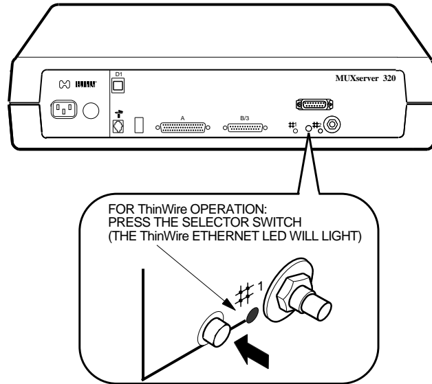
Figure 5–3: Selecting ThinWire Ethernet
